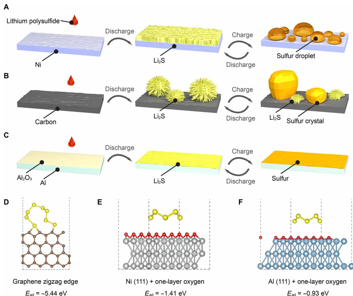
Fig. 2. Schematic of sulfur evolution and mechanism understanding by theoretical calculations. Schematic illustration of the sulfur species evolution on (A) Ni, (B) C, and (C) Al substrates during charging and discharging processes. Adsorption energy and configuration of S 8 adsorbed on (D) graphene zigzag edge, (E) nickel (111) surface covered by one layer of oxygen, and (F) aluminum (111) surface covered by one layer of oxygen.
